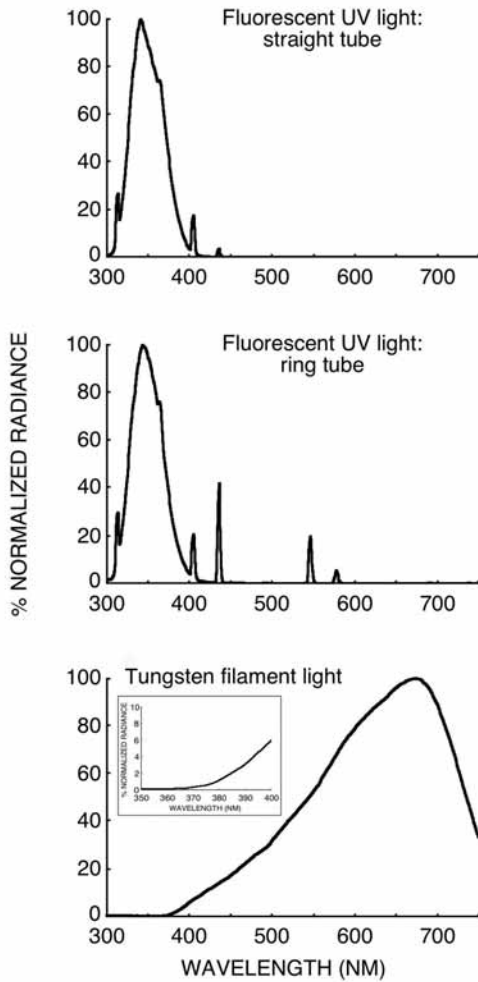
Figure 2. Spectral properties of the output of the three light sources used in UV imaging. The inset for the tungsten filament light source shows its output in the UV with the intensity scale expanded. See text for details.
