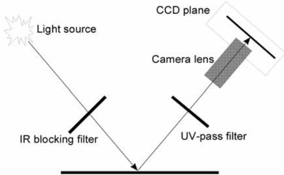
Figure 3. Light path diagram for a typical UV imaging system.
