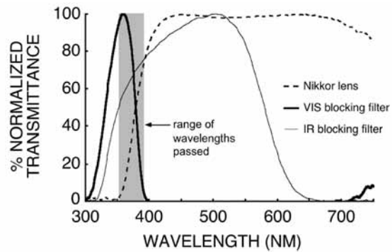
Figure 4. Transmission spectra for elements in the light path used for UV imaging. Shaded range of wavelengths is that that would be passed through a system with these elements. See text for details.
