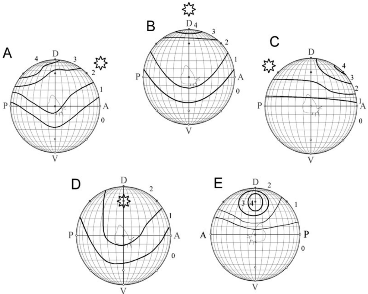
Figure 5. Changes in the number of wings that fully and simultaneously reflected ultraviolet light, as a function of light source location (shown by sunburst icon) and receiver location in the space around a male in flight ( N = 3 ). The light source locations examined were: A, elevation 90^\circ ; azimuth 0^\circ ; B, elevation 45^\circ , azimuth 0^\circ ; C, elevation 45^\circ , azimuth 180^\circ ; D, elevation 45^\circ , azimuth 90^\circ , sample points from animal's left side; E, elevation 45^\circ , azimuth 90^\circ , sample points from animal's right side (light source location not visible). D, dorsal; V, ventral; A, anterior; P, posterior. Numbers of increasing value correspond to isoclines of increasing brightness (i.e. isocline 4 is the brightest; isocline 0 is the least bright).
