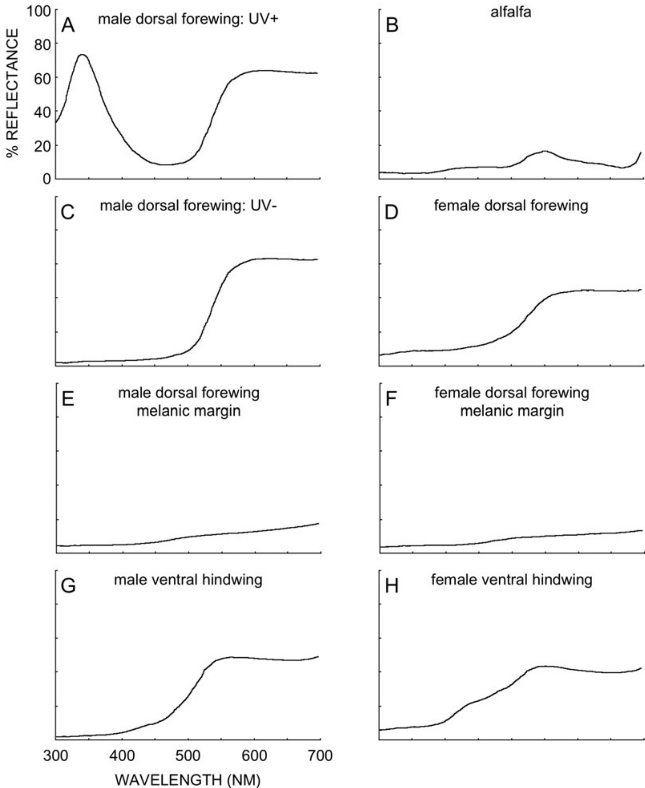
Figure 7. Mean reflectance spectra: A, male dorsal forewing using a spatial arrangement in which ultraviolet (UV) intensity was maximized (UV+); B, alfalfa; C, male dorsal forewing using a spatial arrangement in which UV reflectance was minimized (UV-) orientation; D, female dorsal forewing; E, male melanic margin; F, female melanic margin; G, male ventral hind wing ( N = 26 ); H, female ventral hind wing. Sample size for all, except male ventral hind wing, N = 35 .
