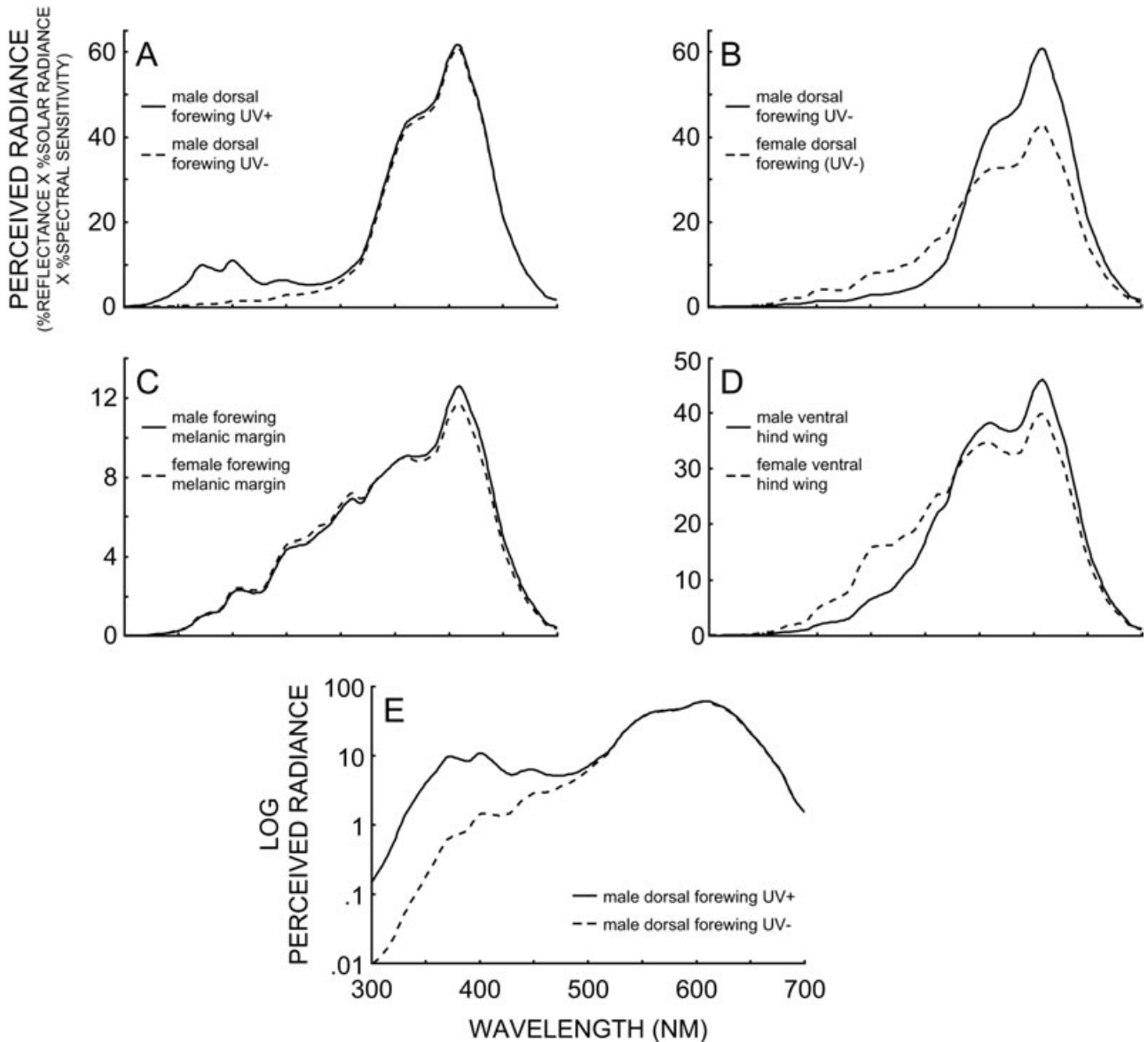
Figure 9. Estimated perceived radiance of wing regions examined in the present study.
