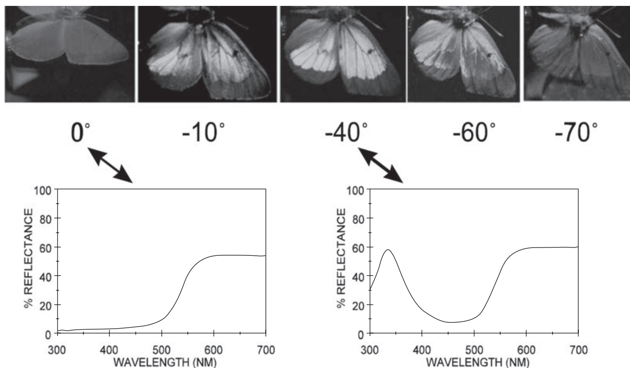
Figure 4. A, changes in appearance in ultraviolet (UV) imaging of male Colias eurytheme wings as they are swept through a down stroke of the wing beat cycle. In this example, the light source was located at elevation 90° and azimuth 0°, and the camera was located at elevation 45° and azimuth 90°. B, reflectance spectra of the wings showing the absence (left) and near maximum (right) reflectance of the iridescent structural UV coloration.
