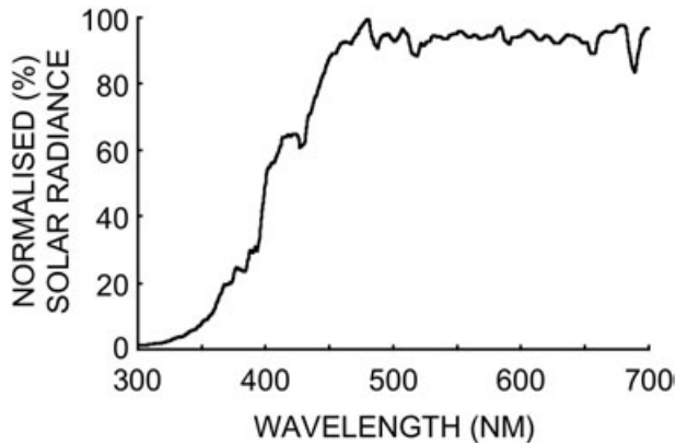
Figure 2. Solar radiance (normalized to wavelength of peak intensity) in a clear, central Arizona sky.
