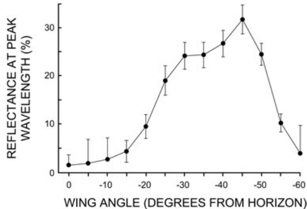
Figure 8. Intensity changes in ultraviolet reflectance peak wavelength (mean \pm standard error) with changes in wing angle ( N = 10 ).
