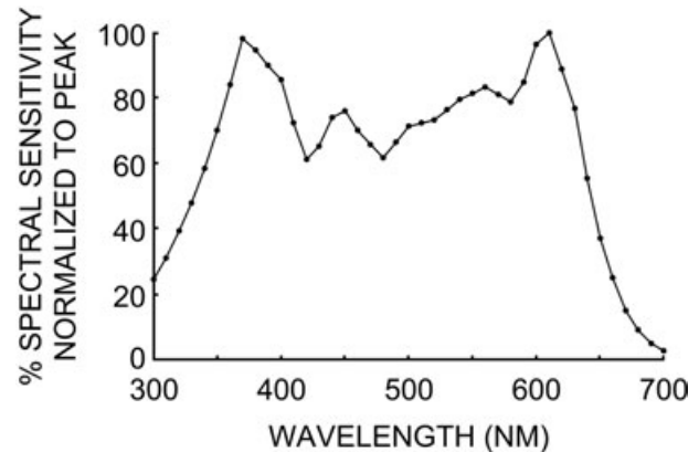
Figure 3. Electroretinograph of Colias eurytheme used to approximate spectral sensitivity in this study. Data summarized from Post & Goldsmith (1969).
