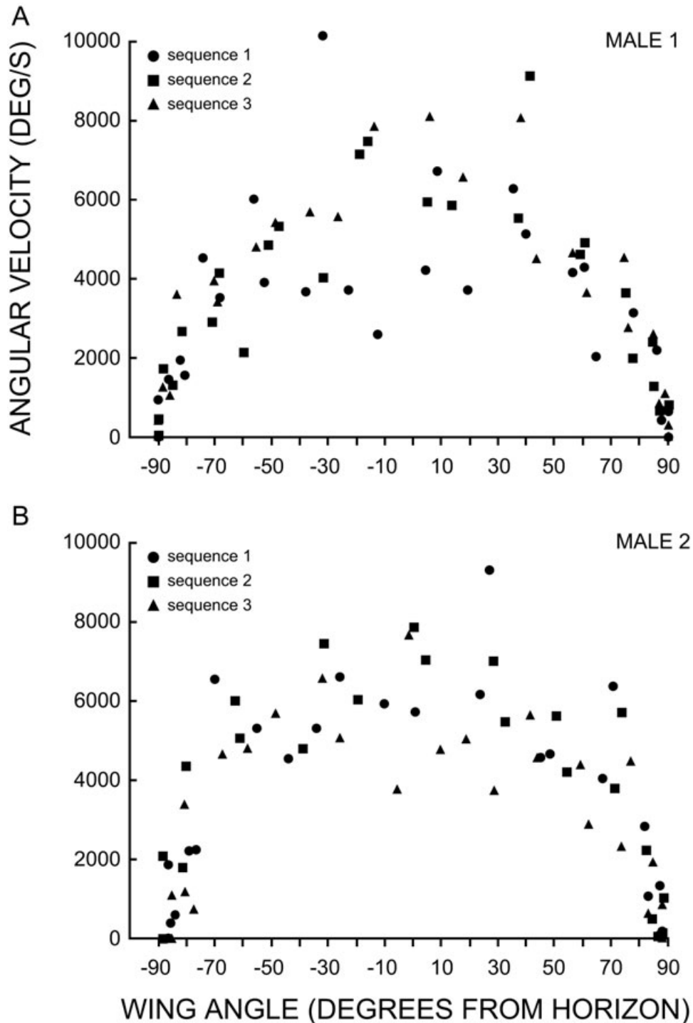
Figure 6. Changes in the angular velocity of the wings during a wing beat. Data are shown for two males and for three full wing beat cycles from each male.
