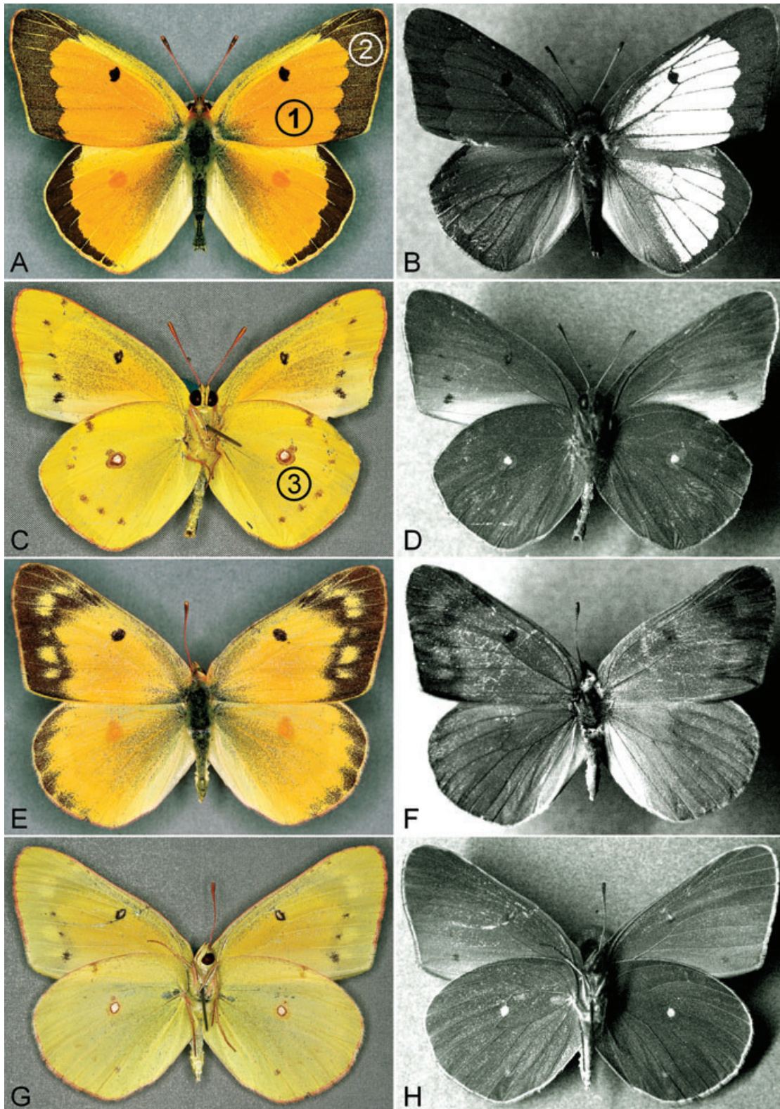
Figure 1. Dorsal and ventral wing surfaces of male and female Colias eurytheme in visible (left panels) and ultraviolet (right panels) light. A, B, male dorsal surface. C, D, male ventral surface. E, F, female dorsal surface. G, H, female ventral surface. In (A) and (C), numbers in circles refer to spectral measurement locations for all specimens: (1) dorsal forewing central orange area, (2) melanic margin, and (3) ventral hind wing.
