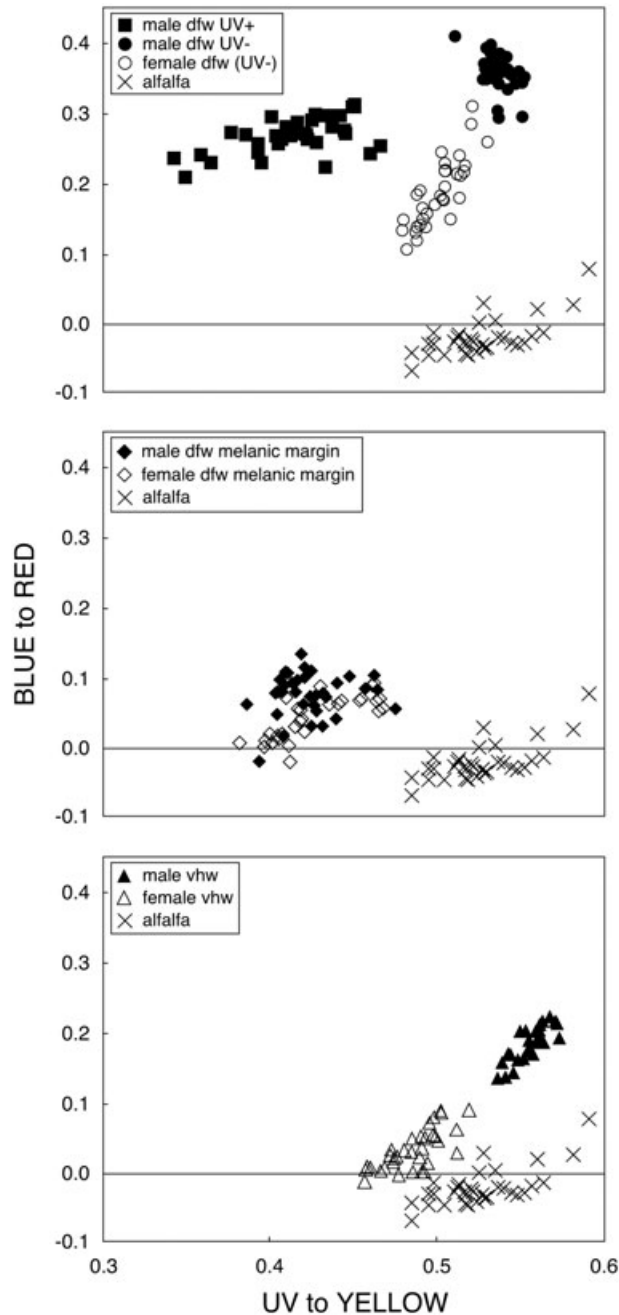
Figure 10. Perceived radiance colour scores plotted in the colour space of Endler (1990). UV, ultraviolet.
